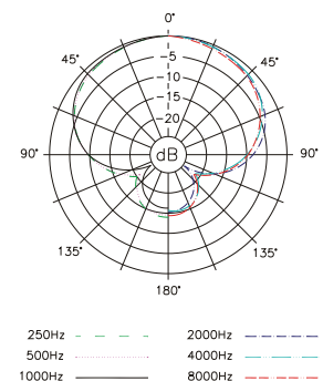
Pick-Up Pattern
